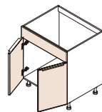
Item: Sink Base Cabinet Code: SB30, SB33, SB36, SB42 H×D: 30" ×24"
