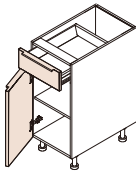
Item: Vanity Base With 1 Door+1 Drawer Code: VB15, VB18, VB21 H×D: 30" ×21 "
