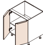
Item: Base Full Door Cabinet Code: B24FD, B27FD, B30FD B33FD, B36FD H×D: 30" ×24"
