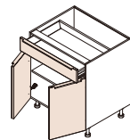
Item: Base Cabinet Code: B24, B27, B30, B33, B36, B42 H×D: 30" ×24"
