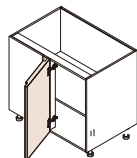
Item: Base Blind Corner Cabinet Code: BBC36-42 (36Carcass+15Door) BBC36-45 (36Carcass+18Door) BBC42-45 (42Carcass+18Door) H×D: 30" ×24"
