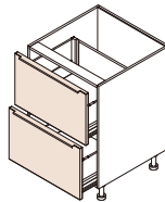
Item: Vanity Base With 2 Drawers Code: VD12-2, VD15-2, VD18-2 VD21-2, VD24-2 H×D: 30" ×21 "
